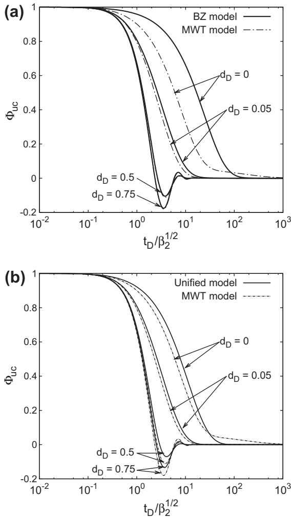
Fig. 5. Semi-log plots of dimensionless head, \Phi_{uc}(t_D) , against dimensionless time, t_D/\sqrt{\beta_2} , for different depths ( d_D ) below the water table, comparing the MWT solution to (a) the confined aquifer (BZ) solution of Butler and Zhan (2004) and (b) the unified model.
